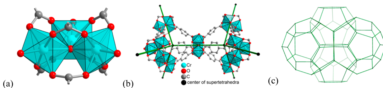
Figure 1. MIL-101Cr network with the (a) trinuclear \{Cr_3(\mu_3-O)(O_2C-)_6(F,OH)(H_2O)_2\} building unit which forms the vertices of supertetrahedra (b). Vertex-sharing supertetrahedra (b) then form two types of mesoporous cages with pentagonal and hexagonal windows (c). For presentation of the pore and window size see Figure S1, Supporting Information.
