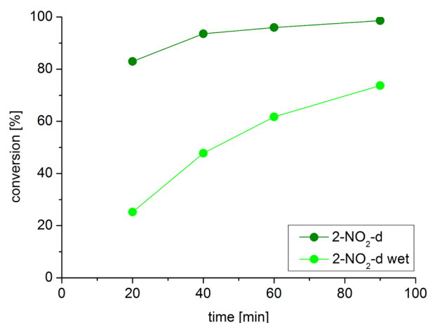
Figure 7. Activity of 2-NO 2 -d after an additional wetting with water.
